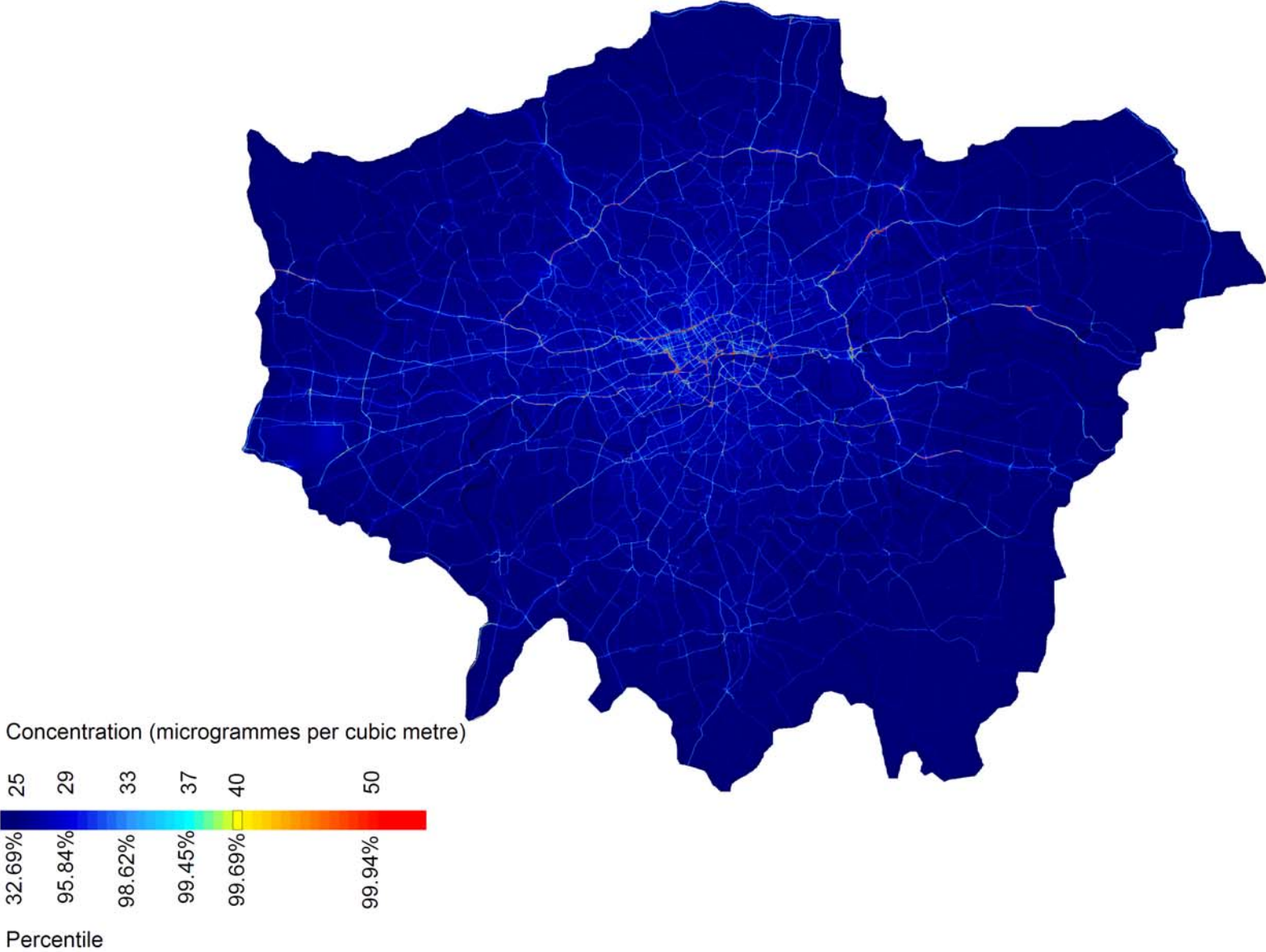
Modelled 2004 Annual Mean PM10 Concentration (microgrammes per cubic metre), based on 2003 Meteorology and the LAEI 2004
